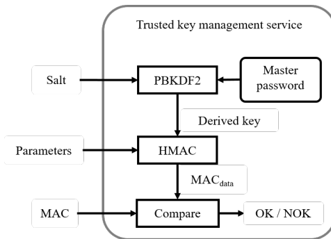
Figure 3: Process overview of authenticating requests from the key management client in the trusted key management service.
