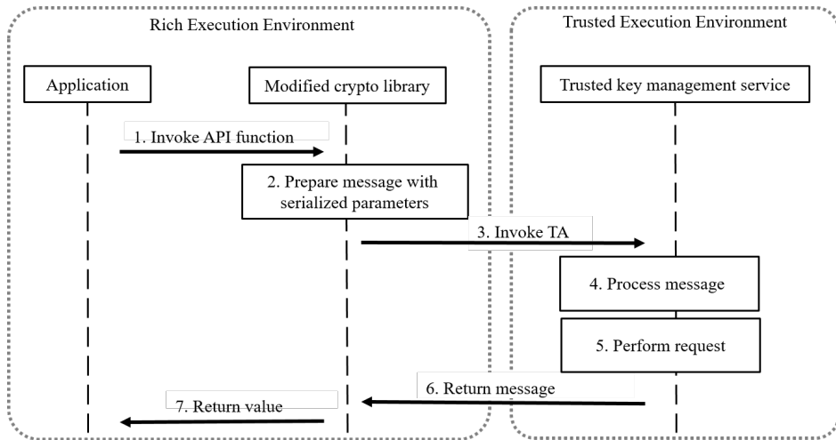
Figure 4: Interactions involved in performing cryptographic operations with private keys stored and managed in the TEE.
