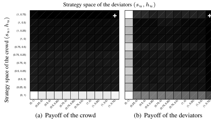
Figure 2. Simulation results in the random walk model (darker means higher payoff)
