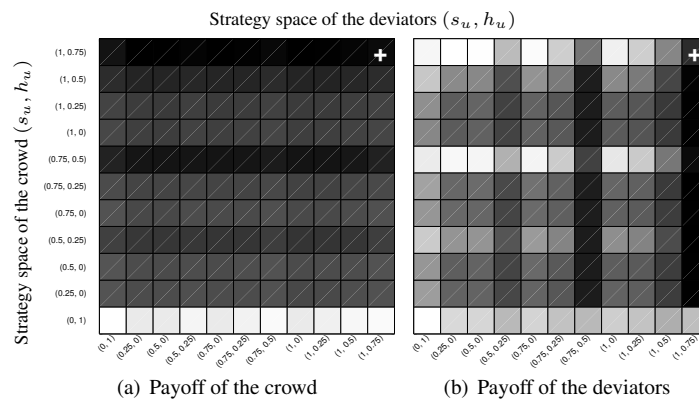
Figure 3. Simulation results in the grid-based random waypoint model (darker means higher payoff)
