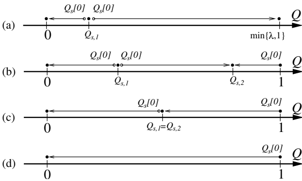
Fig. 2. Dynamics of SCO for \lambda < 2 and \beta \geq \frac{2}{2-\lambda} \alpha : (a) 0 < P_s \leq \beta - \frac{1}{\lambda}(\beta - \alpha) , (b) \beta - \frac{1}{\lambda}(\beta - \alpha) < P_s < \frac{\beta^2 \lambda}{4(\beta - \alpha)} , (c) P_s = \frac{\beta^2 \lambda}{4(\beta - \alpha)} , (d) P_s > \frac{\beta^2 \lambda}{4(\beta - \alpha)} .
